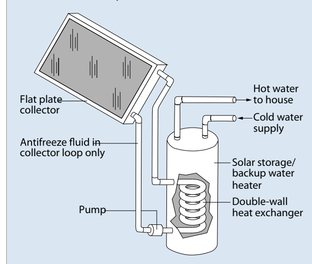
Figure 2. Active, Closed Loop Solar Water Heater. (Photo: U.S. Department of Energy - Office of Energy Efficiency and Renewable Energy)
