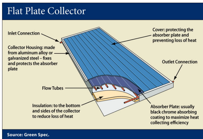
Figure 1. Flat-Plate Collector. (Photo: U.S. Department of Energy)
